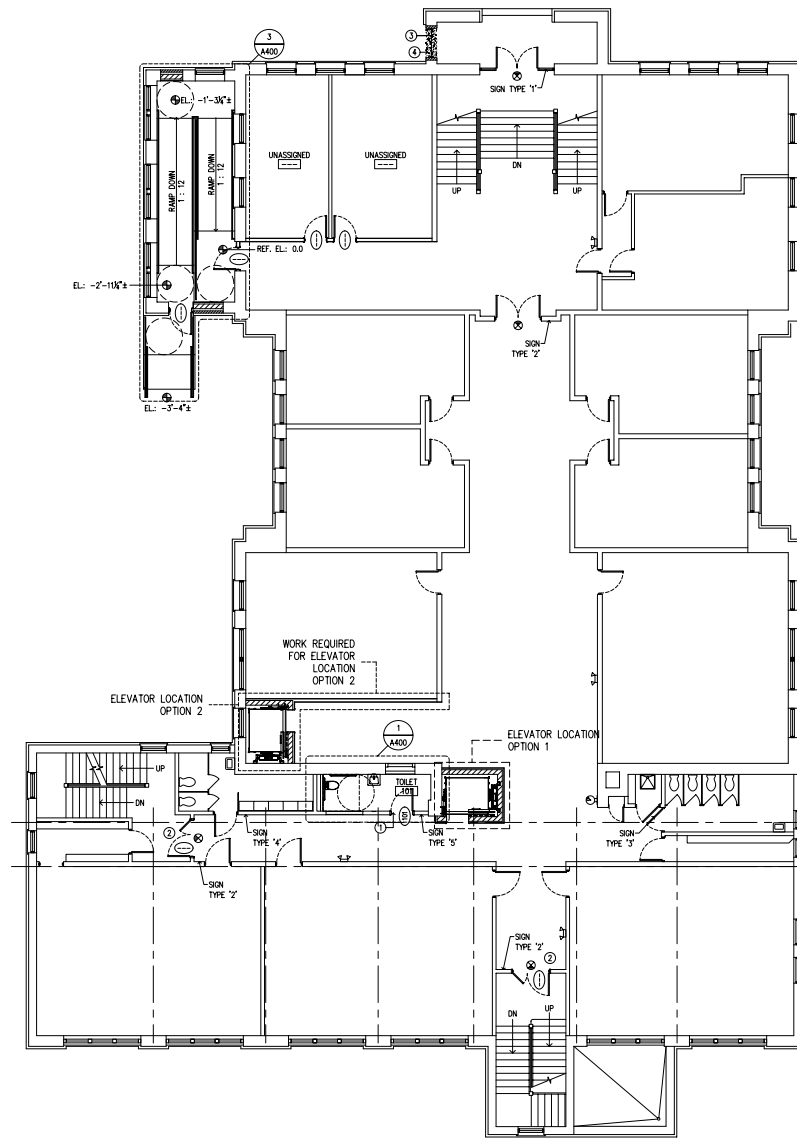
FIRST FLOOR NEW WORK PLAN SCALE: 1/8"=1'-0"
