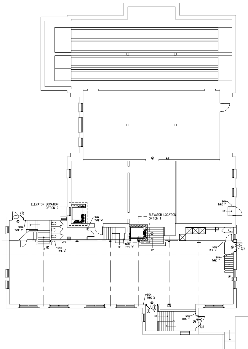
GROUND FLOOR NEW WORK PLAN SCALE: 1/8"=1'-0"
