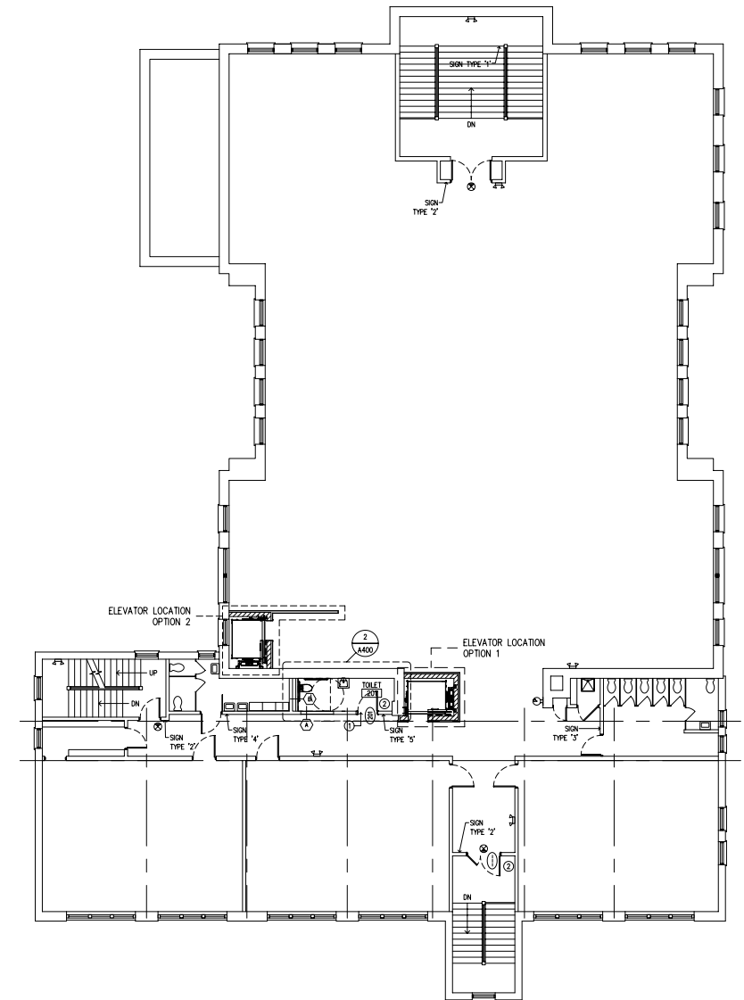
SECOND FLOOR NEW WORK PLAN SCALE: 1/8"=1'-0"
