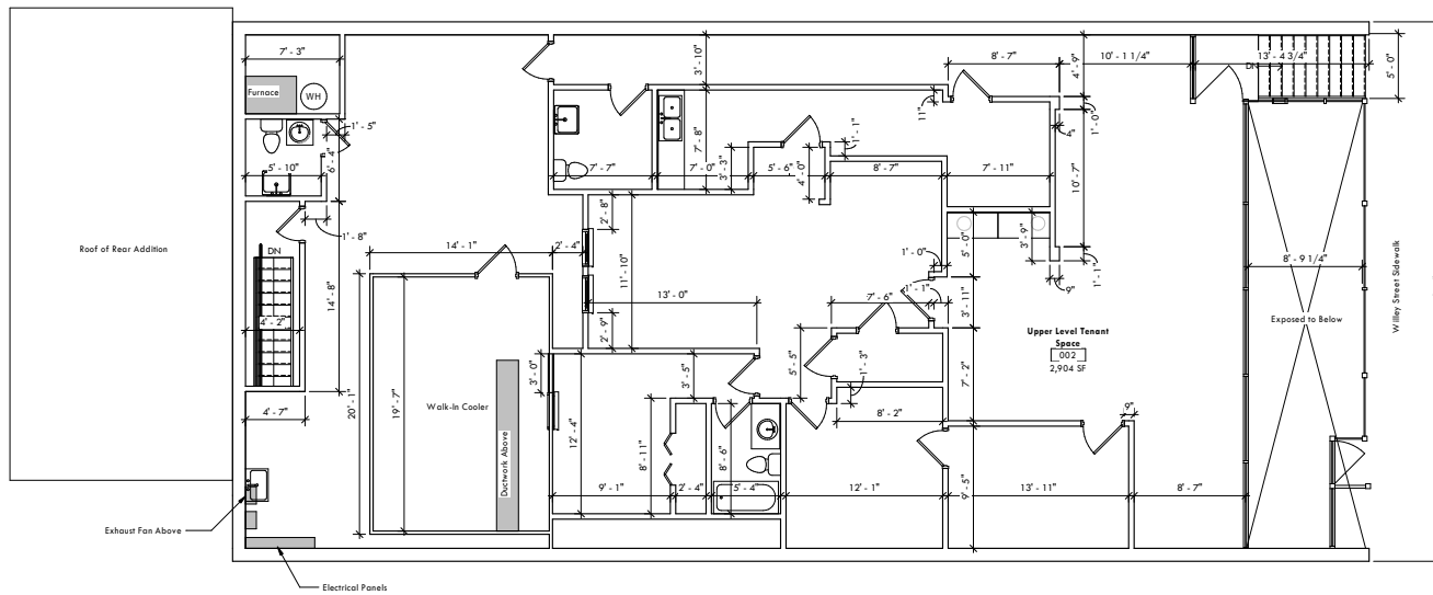
02 - Second Floor - Existing 3/16" = 1'-0"
