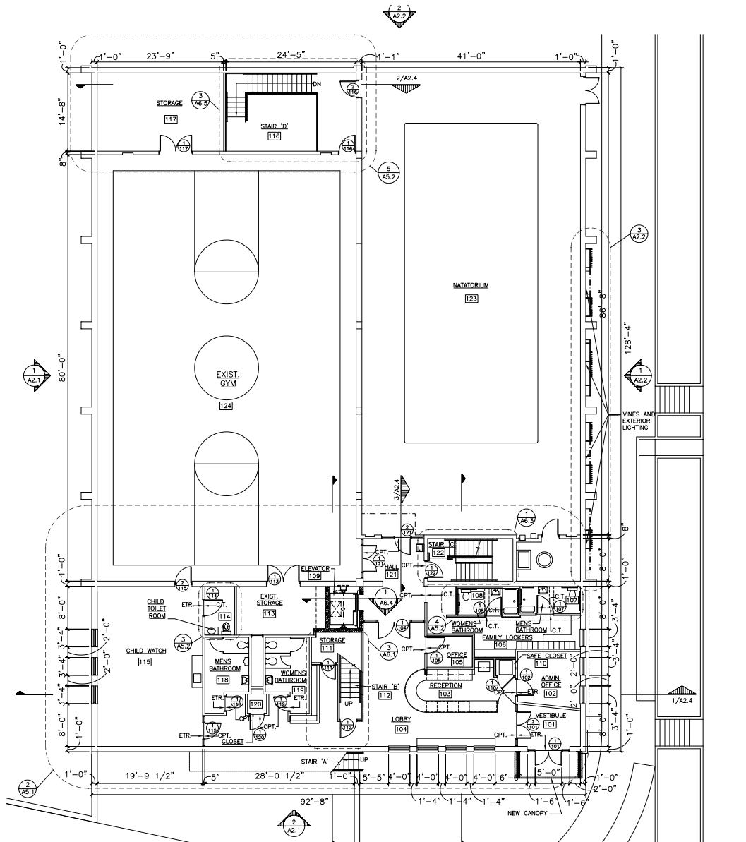
2 FIRST FLOOR PLAN A1.1 1/8"=1'-0"
