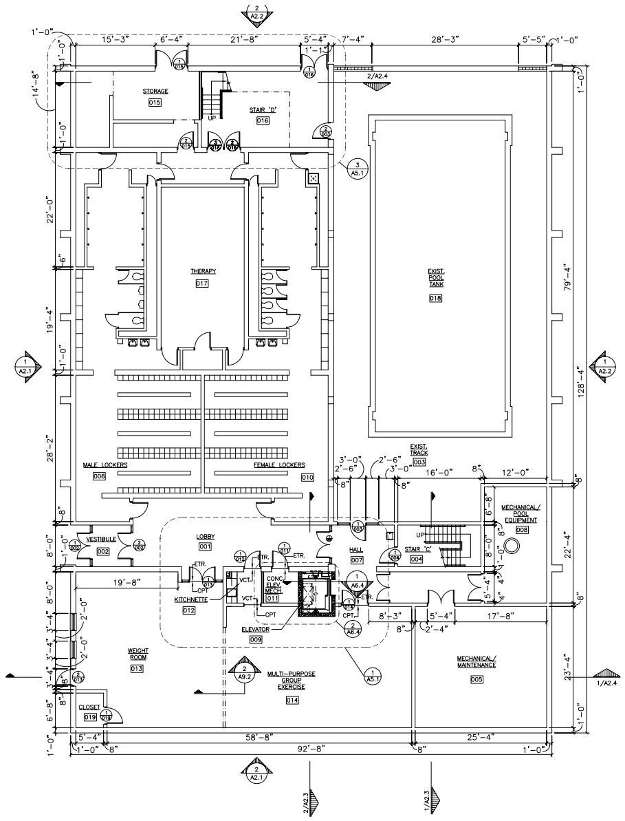
1 BASEMENT FLOOR PLAN A1.1 1/8"=1'-0"
