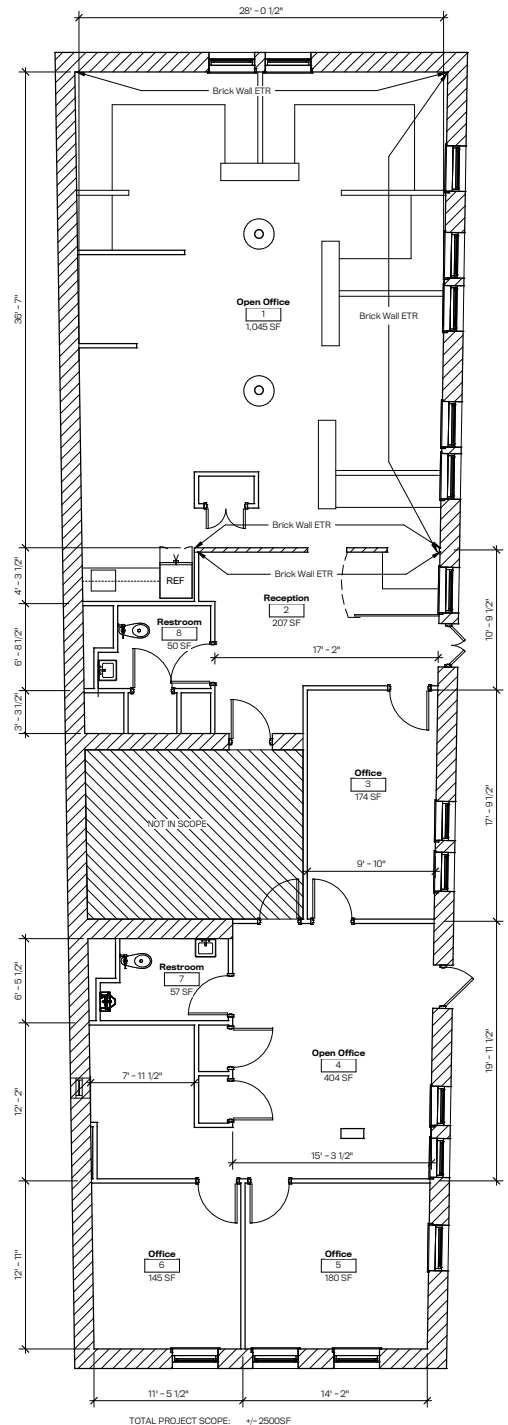
① Second Floor Existing Plan 3/16" = 1'-0"
